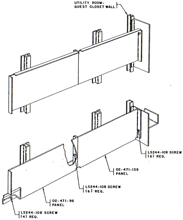
DETAIL "A" STEP N° 10 PAGE N° EM-02-P-31.1
