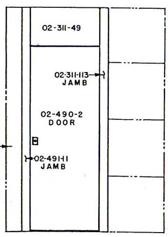
(26) ELEVATION-INSIDE BATH ROOM
