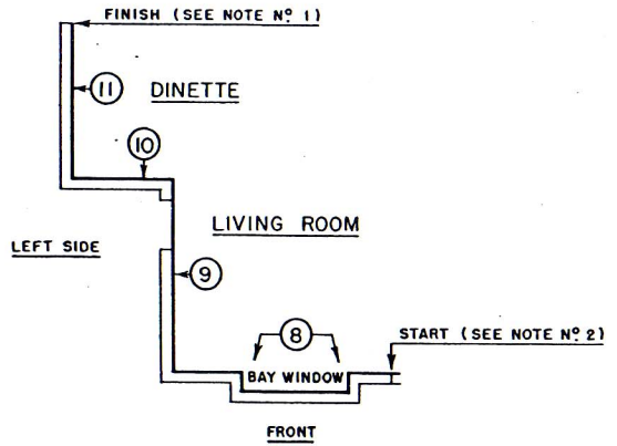
PLAN SHOWING PANEL INSTALLATION PROCEDURE
