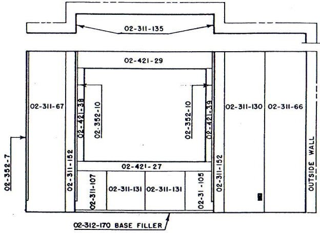
⑧ FRONT ELEVATION - LIVING ROOM
