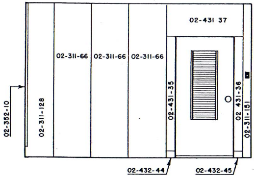
⑨ LEFT SIDE ELEVATION - LIVING ROOM
