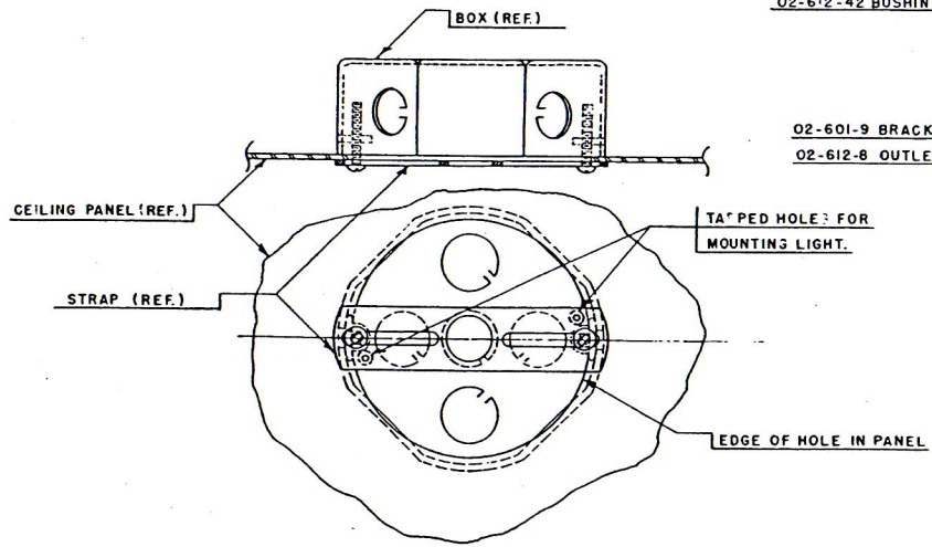
TYPICAL INSTALLATION FOR ALL CEILING FIXTURES.
