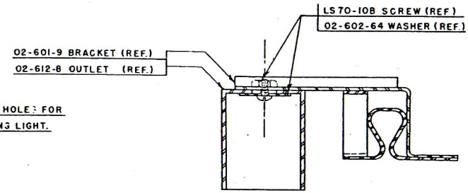
TYPICAL INSTALLATION FOR EXTERIOR & HALL FIXTURES.
