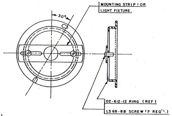
TYPICAL INSTALLATION FOR EXTERIOR & HALL FIXTURES.
