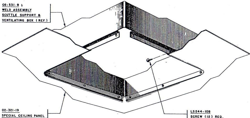
CEILING PANEL TO SCUTTLE BOX ATTACHMENT O2-531-8 SCUTTLE COVER PANEL ASSEM. INSTALLED IN THIS AREA.
