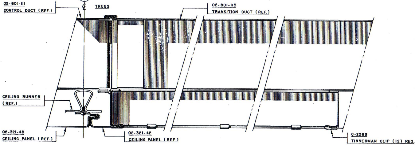
LONGITUDINAL SECTION DUCT TO CEILING PANEL ATTACHMENT
